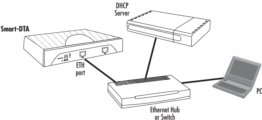
Figure 1. Connecting the Smart-DTA to the network via a hub or switch
